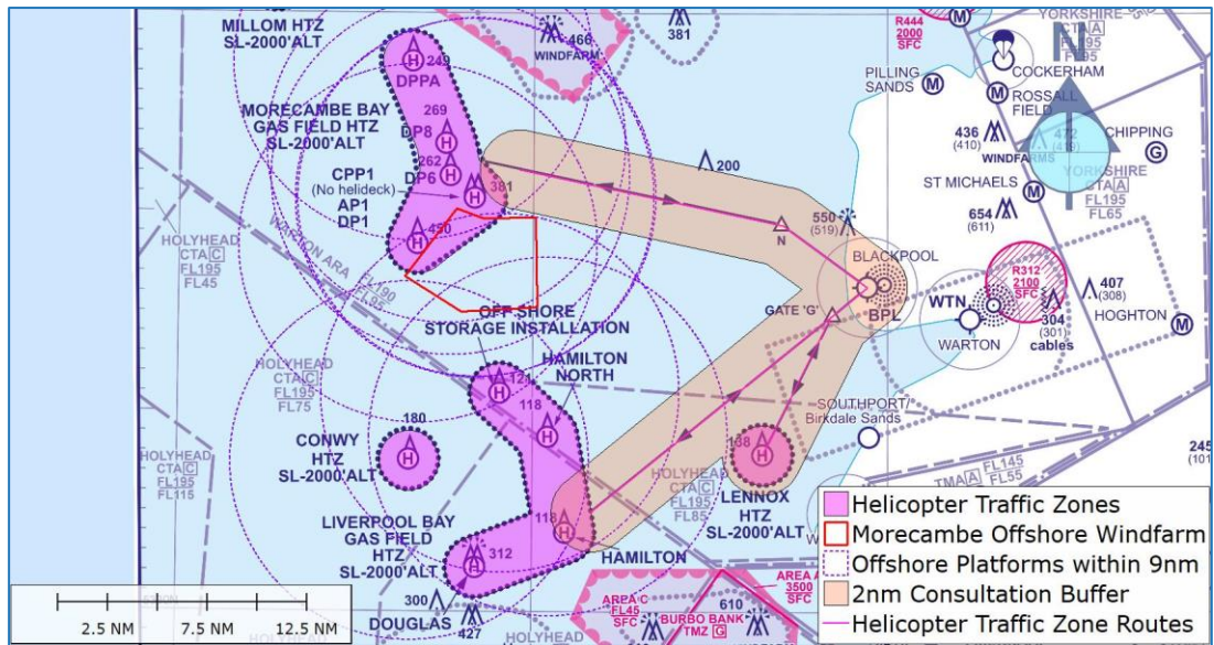
Figure 6: Platforms within 9nm and Helicopter Traffic Zones
