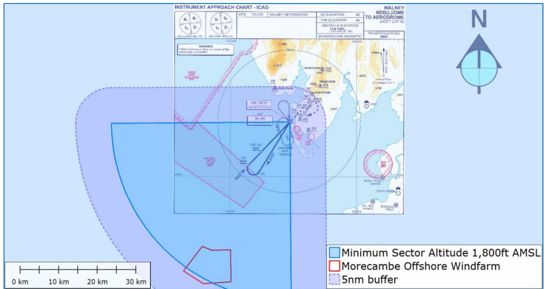
Figure 9: Walney Instrument Approach Chart – NDB(L)/DME To Aerodrome
